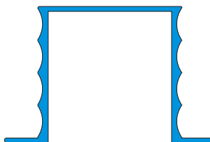
Stand-off bracket #9999
